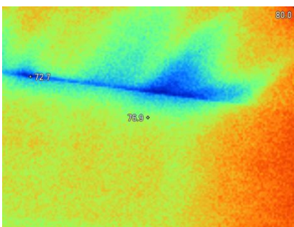
Insulation test
